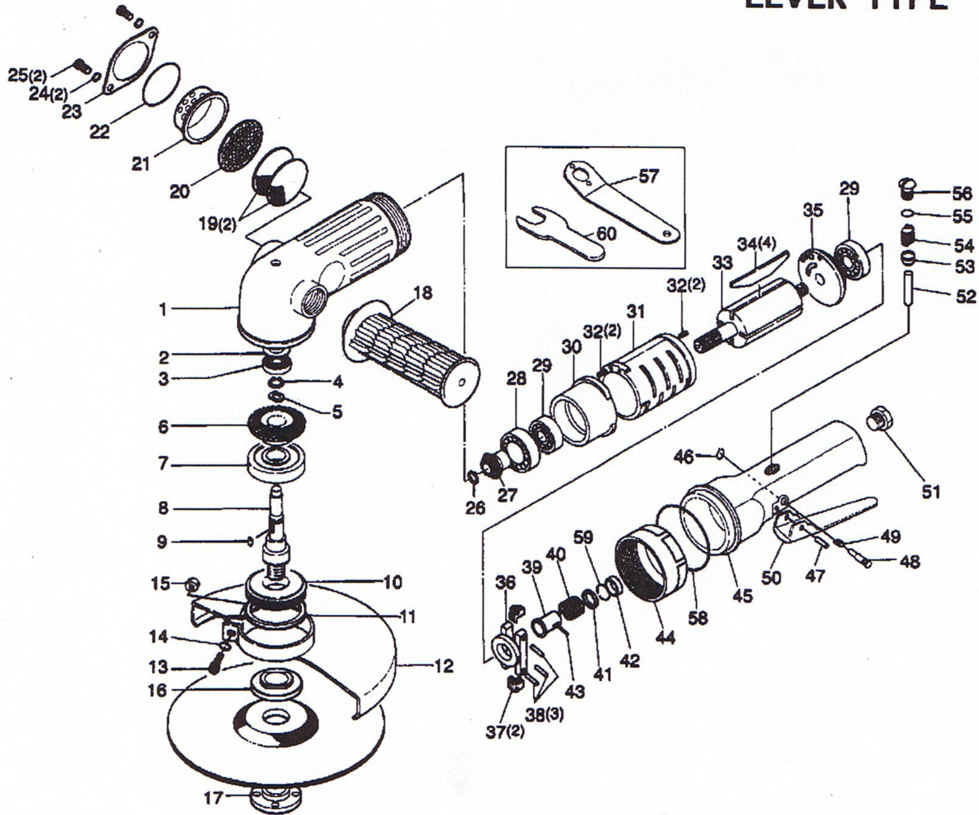
EXPLODED VIEW
